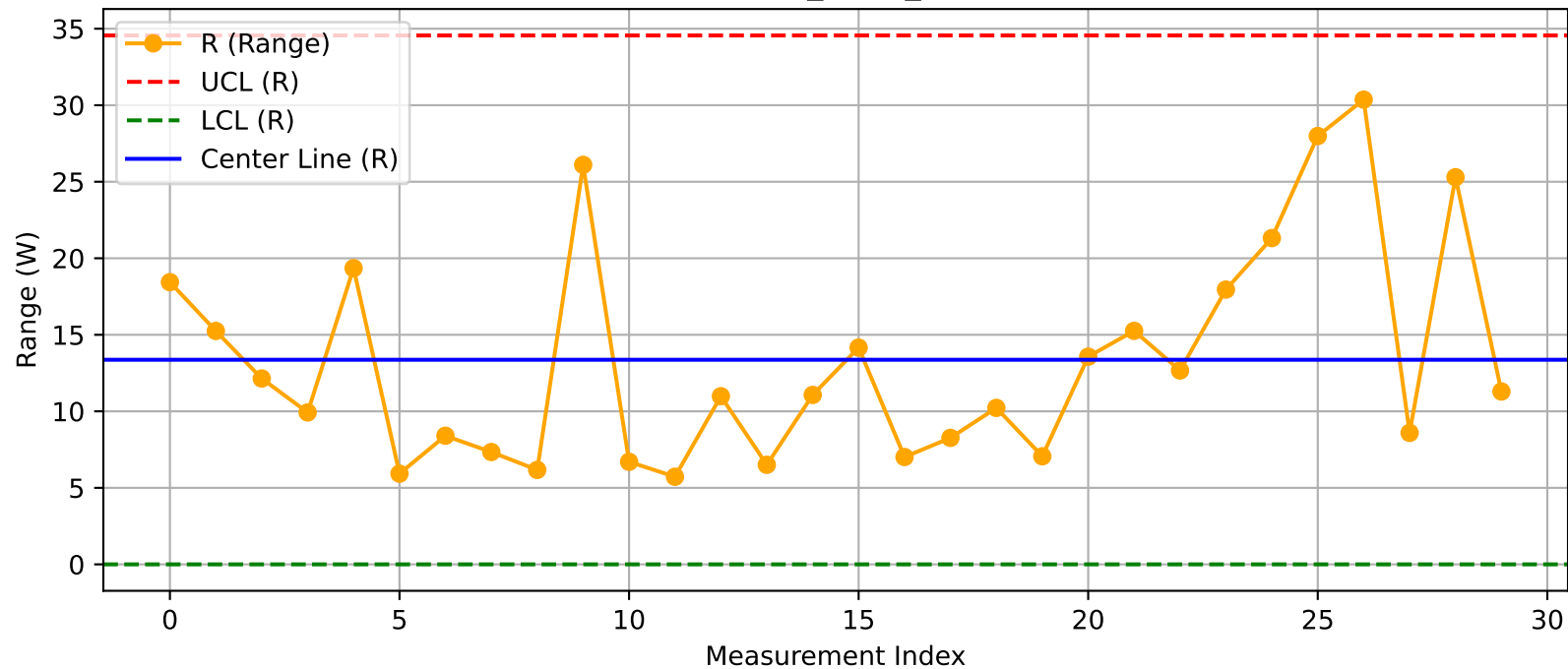
DUT - R Chart (T44_Test1_Xint@Test.xlsx)
