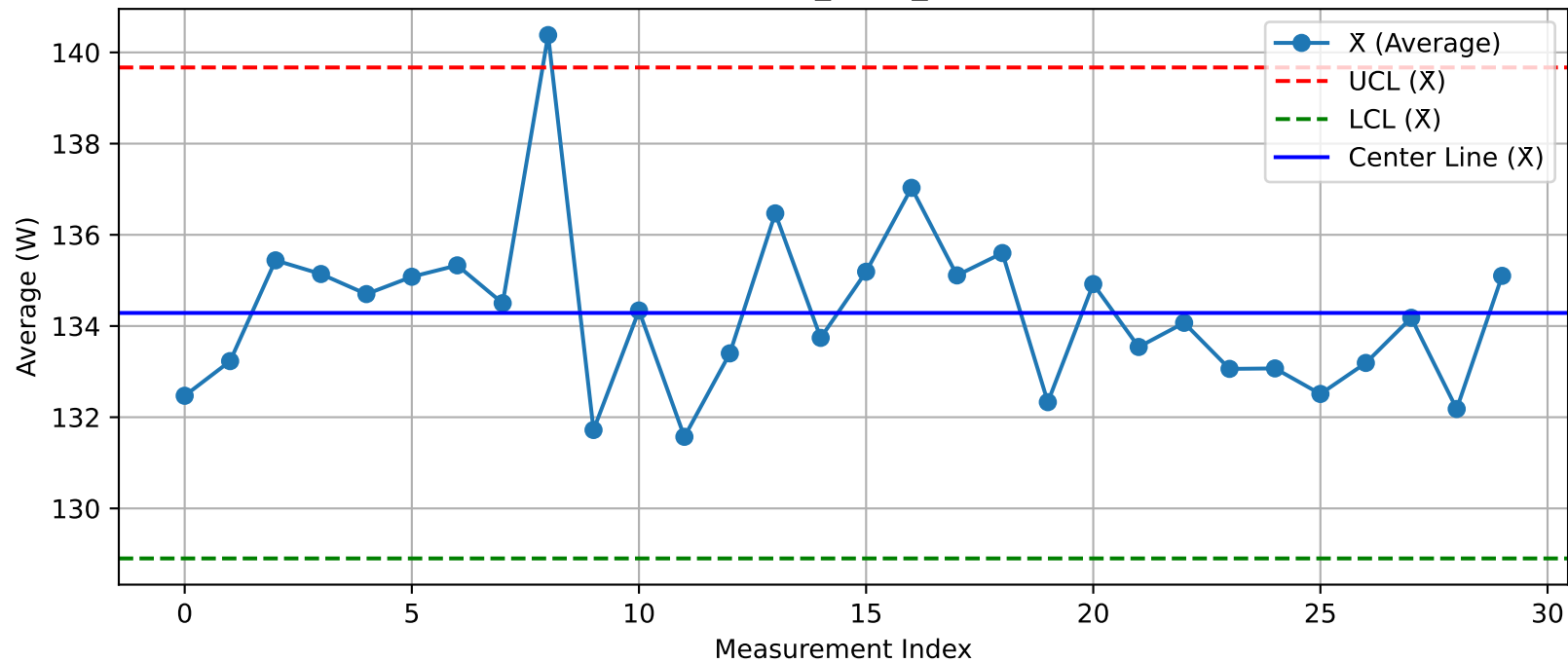
DUT - \bar{X} Chart (T44_Test1_Xint@Test.xlsx)
