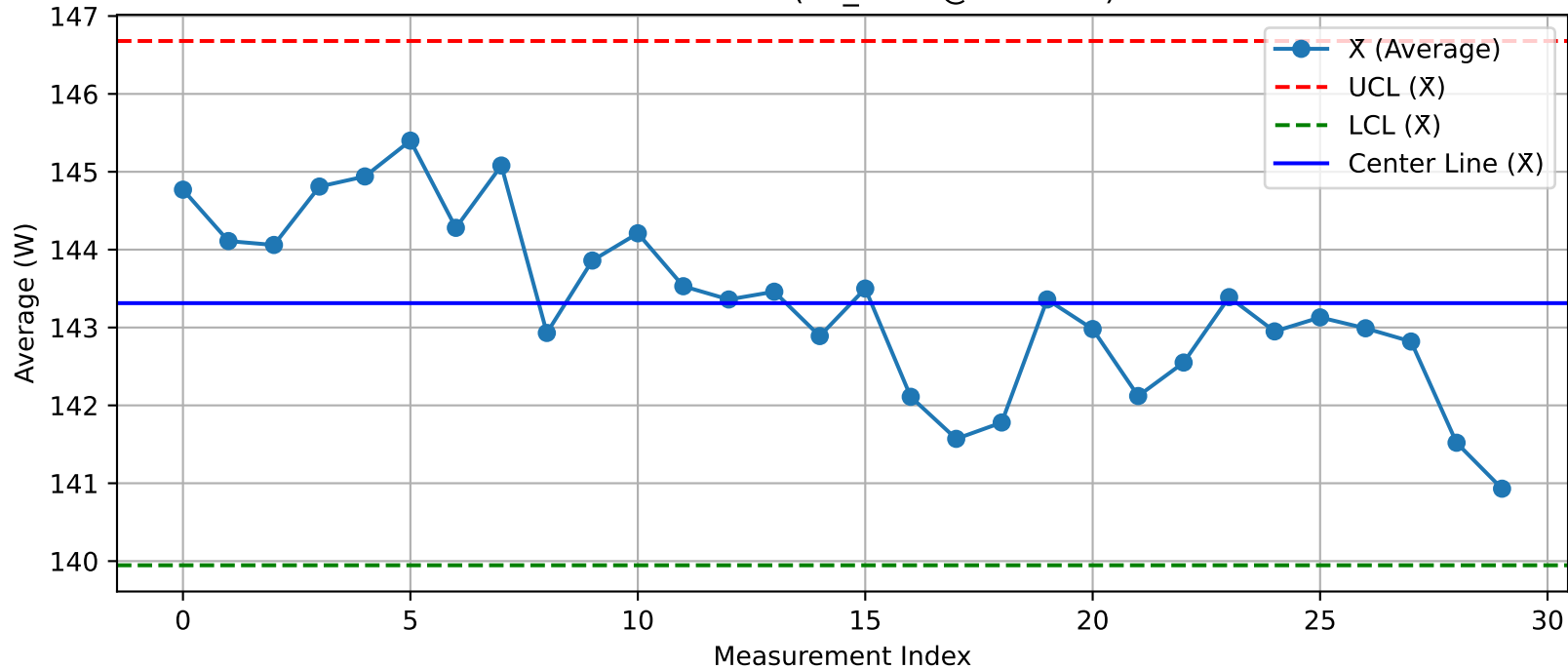
DUT - \bar{X} Chart (T4_Test2@Test.xlsx)
