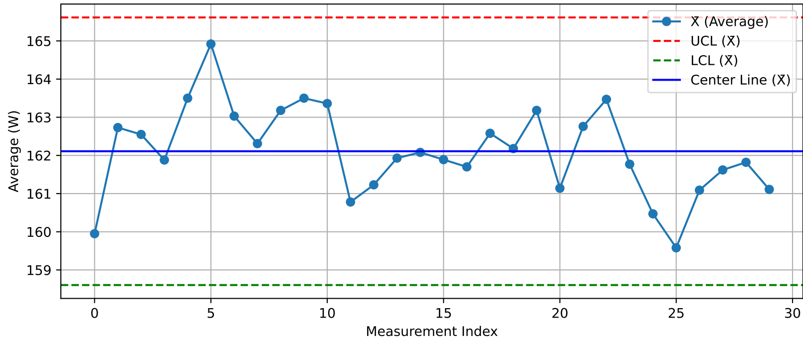
DUT - \bar{X} Chart (T50_Test1_Xint@Test.xlsx)
