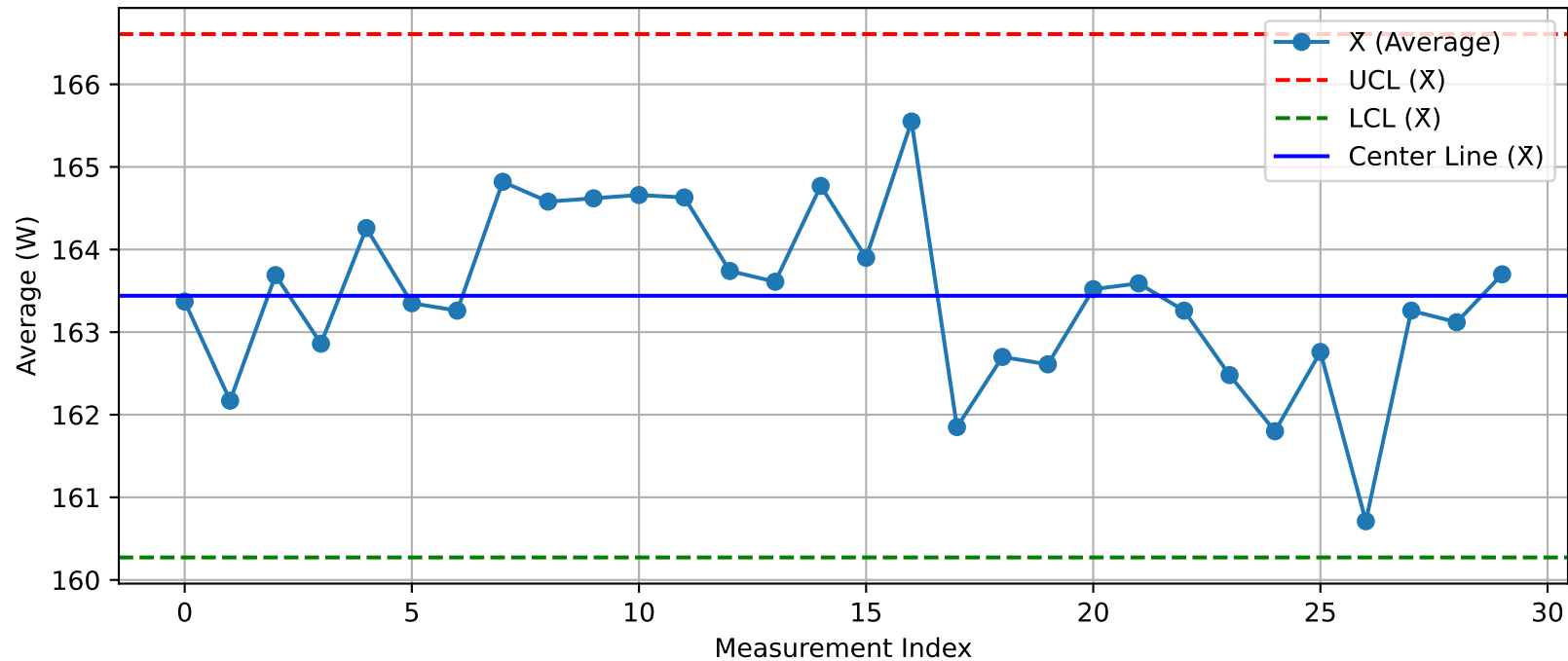
DUT - X Chart (T50_Test2_Xint@Test.xlsx)
