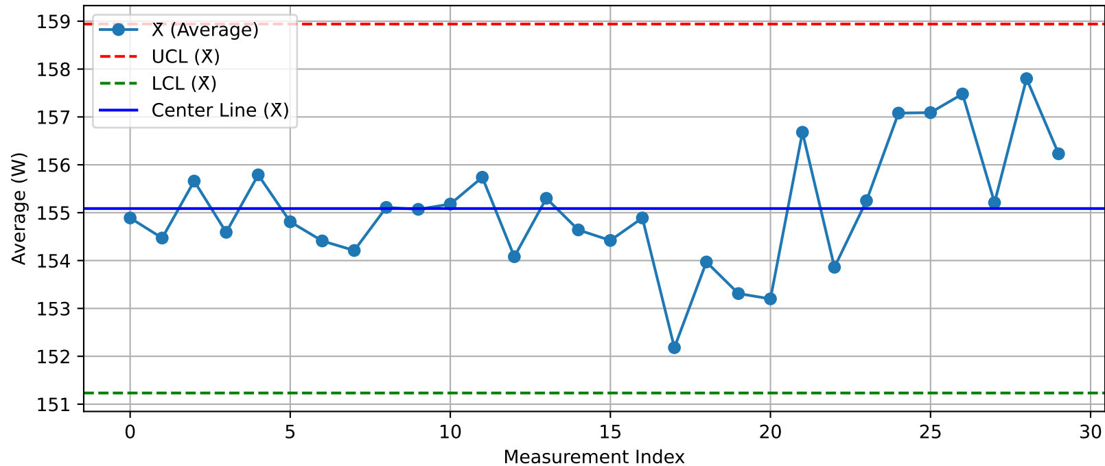
DUT - X Chart (T51_Test1_Xint@Test.xlsx)
