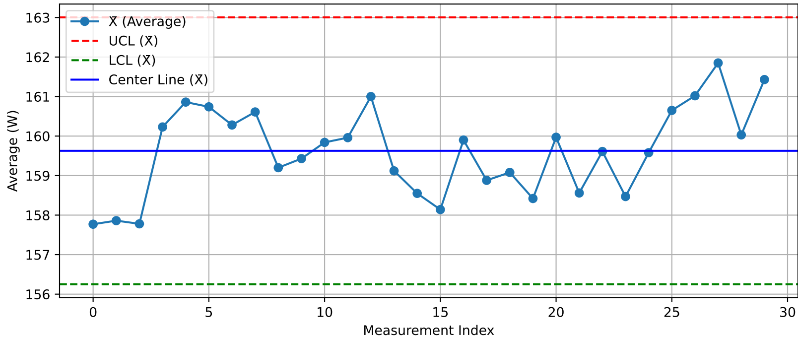
DUT - \bar{X} Chart (T5_Test1@Test.xlsx)
