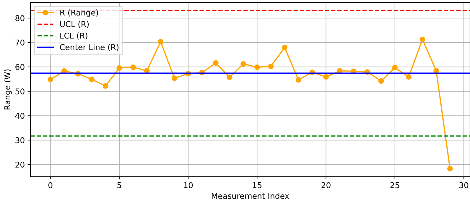
DUT - R Chart (T5_Test1_Xint@Test.xlsx)
