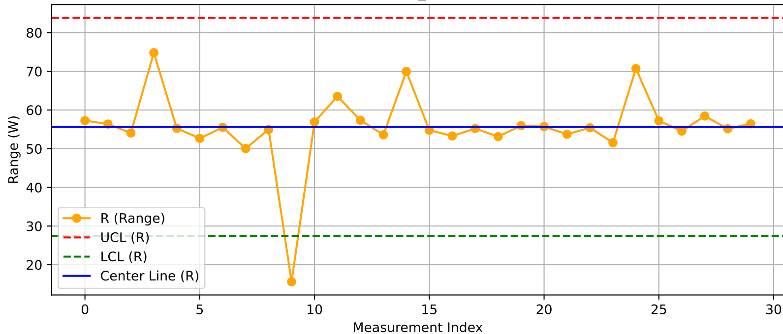
DUT - R Chart (T8_Test1@Test.xlsx)
