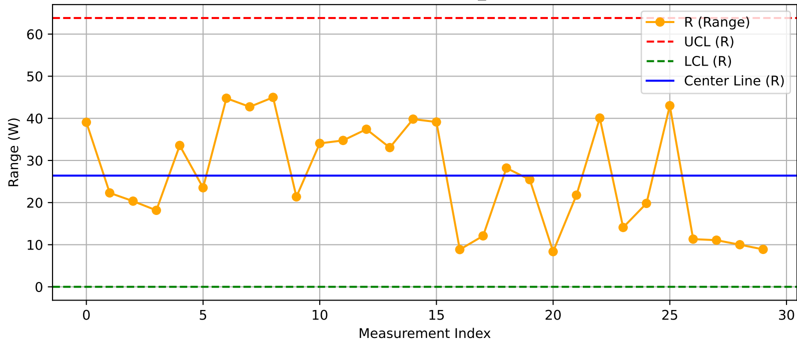
DUT - R Chart (T10@Test1_Nuitka.xlsx)
