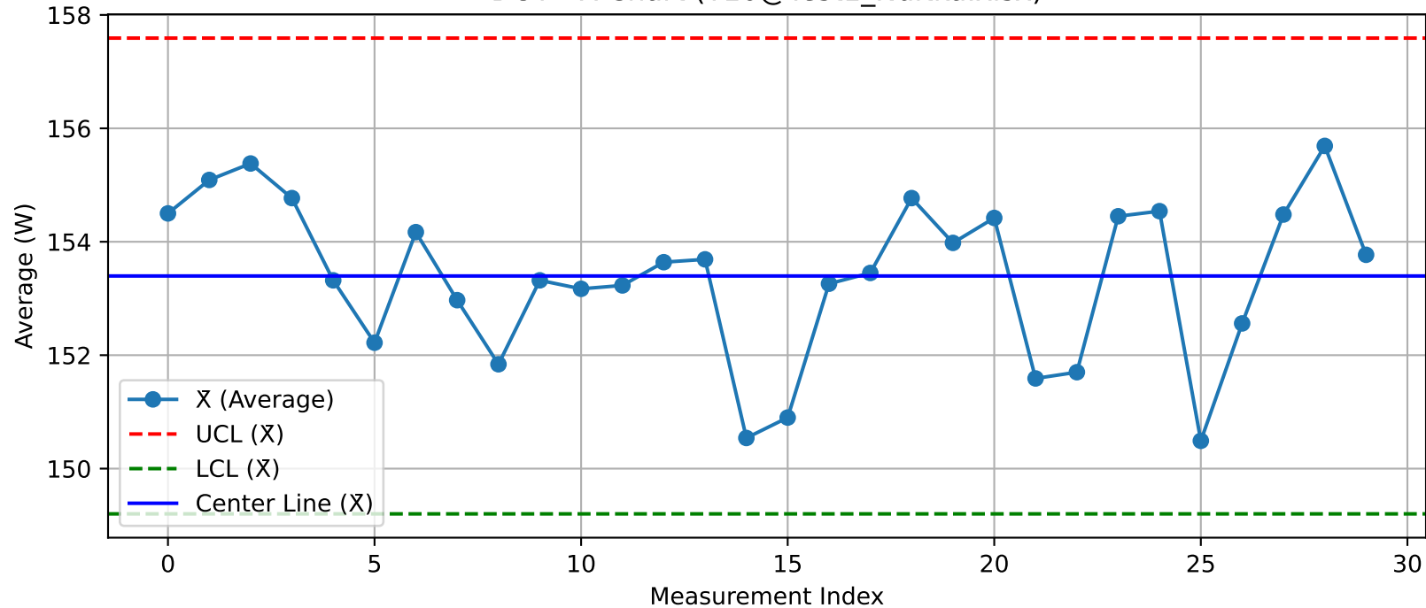
DUT - \bar{X} Chart (T10@Test1_Nuitka.xlsx)
