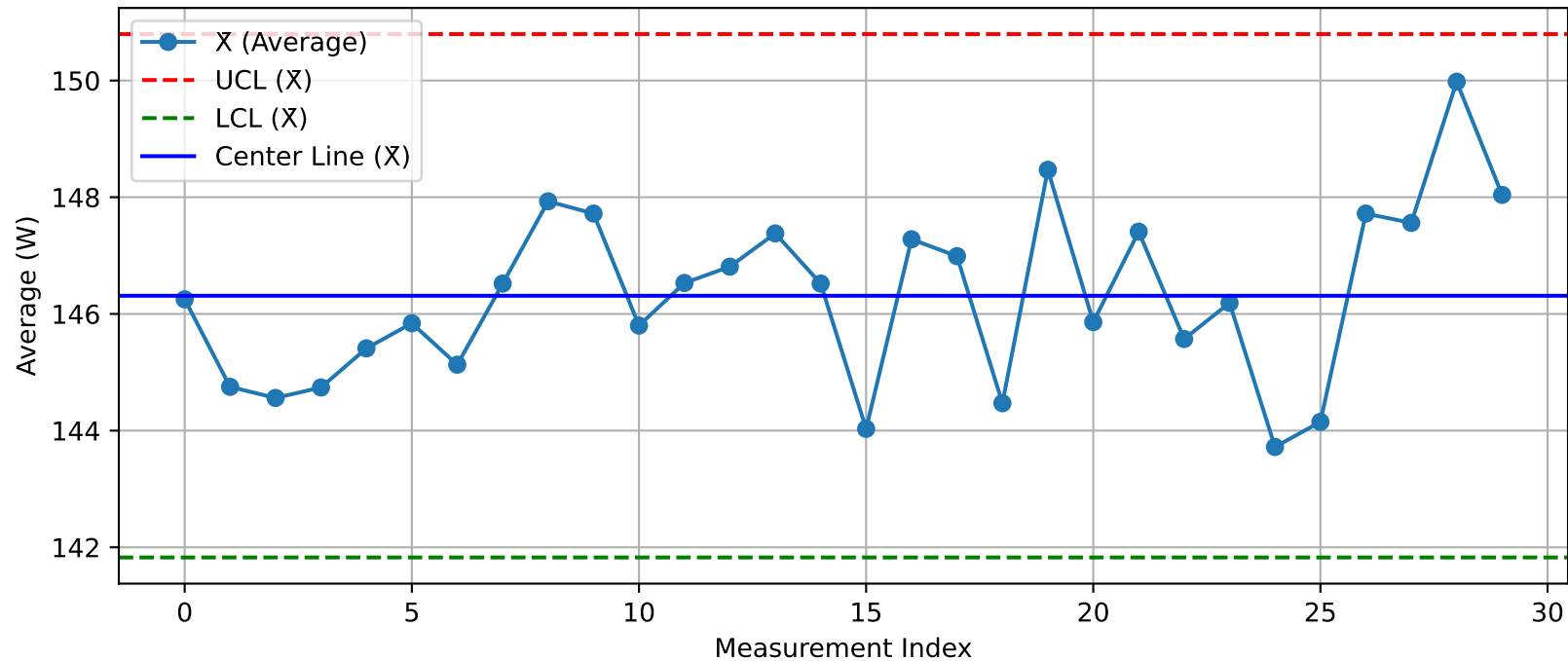
DUT - \bar{X} Chart (T10@Test2_Nuitka.xlsx)
