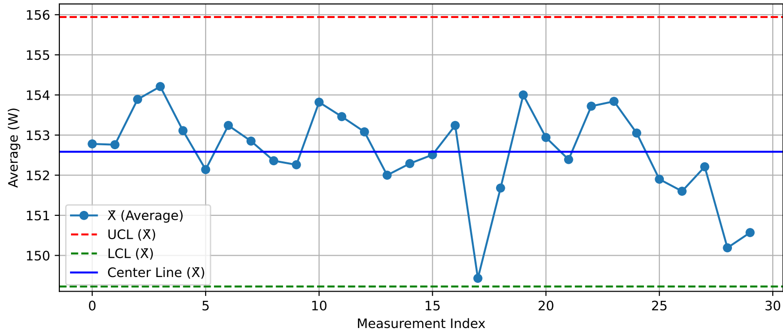
DUT - \bar{X} Chart (T11@Test1_Nuitka.xlsx)
