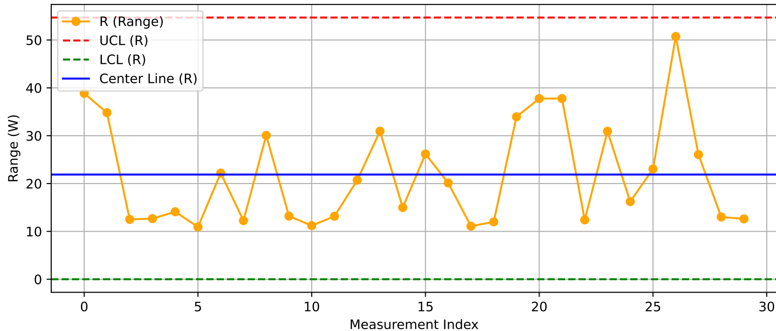
DUT - R Chart (T11@Test2.xlsx)
