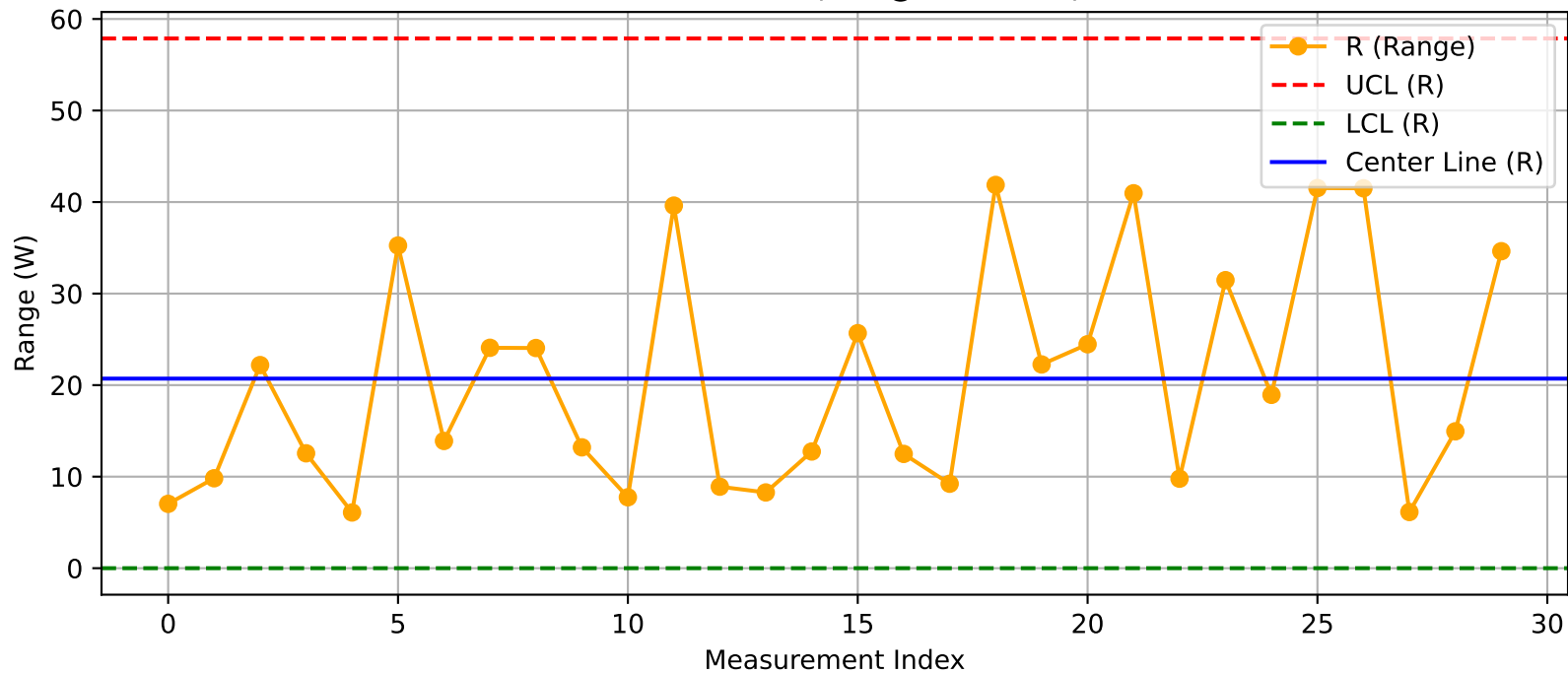
DUT - R Chart (T12@Test2.xlsx)
