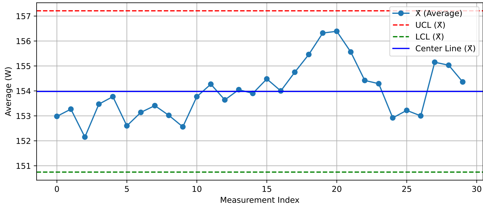
DUT - \bar{X} Chart (T13@Test1.xlsx)
