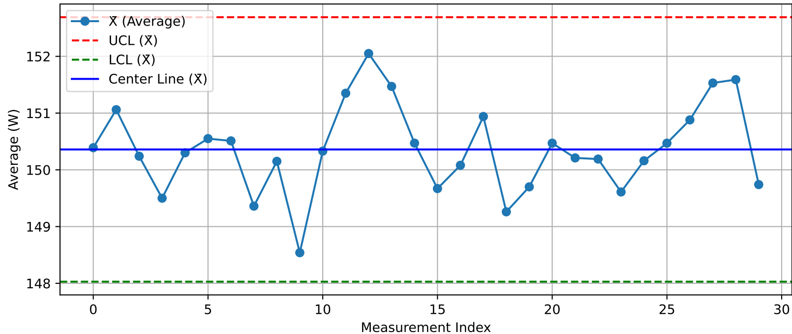
DUT - \bar{X} Chart (T13@Test1_Nuitka.xlsx)
