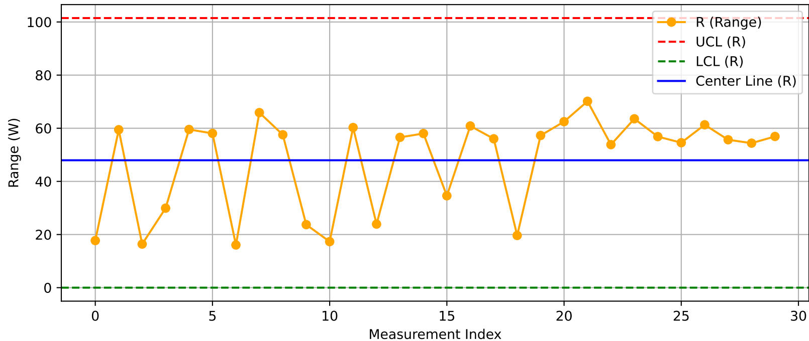
DUT - R Chart (T13@Test2.xlsx)
