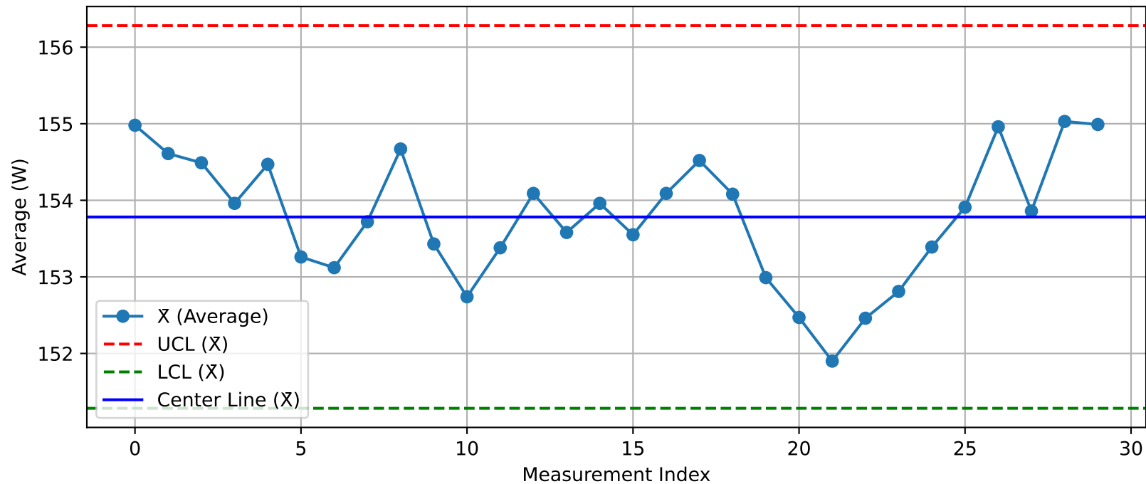
DUT - \bar{X} Chart (T13@Test2.xlsx)
