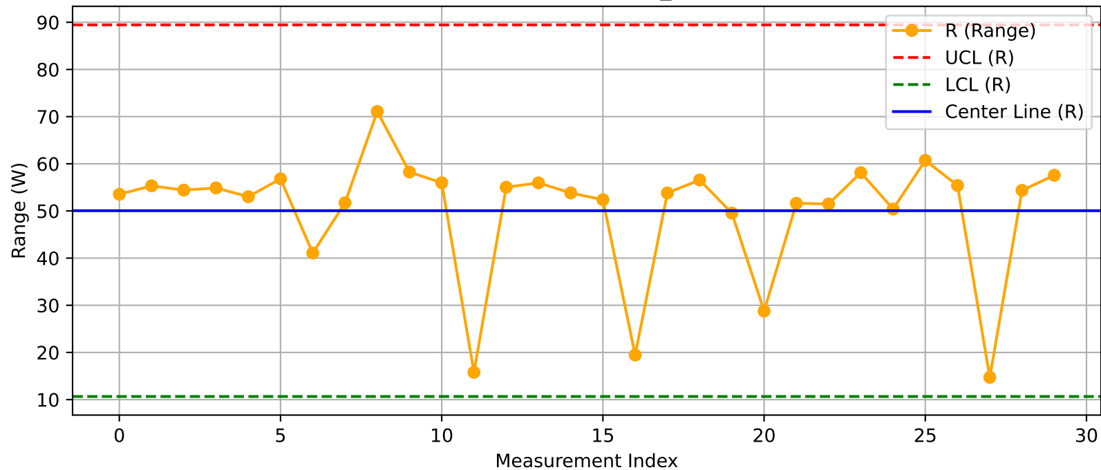
DUT - R Chart (T13@Test2_Nuitka.xlsx)
