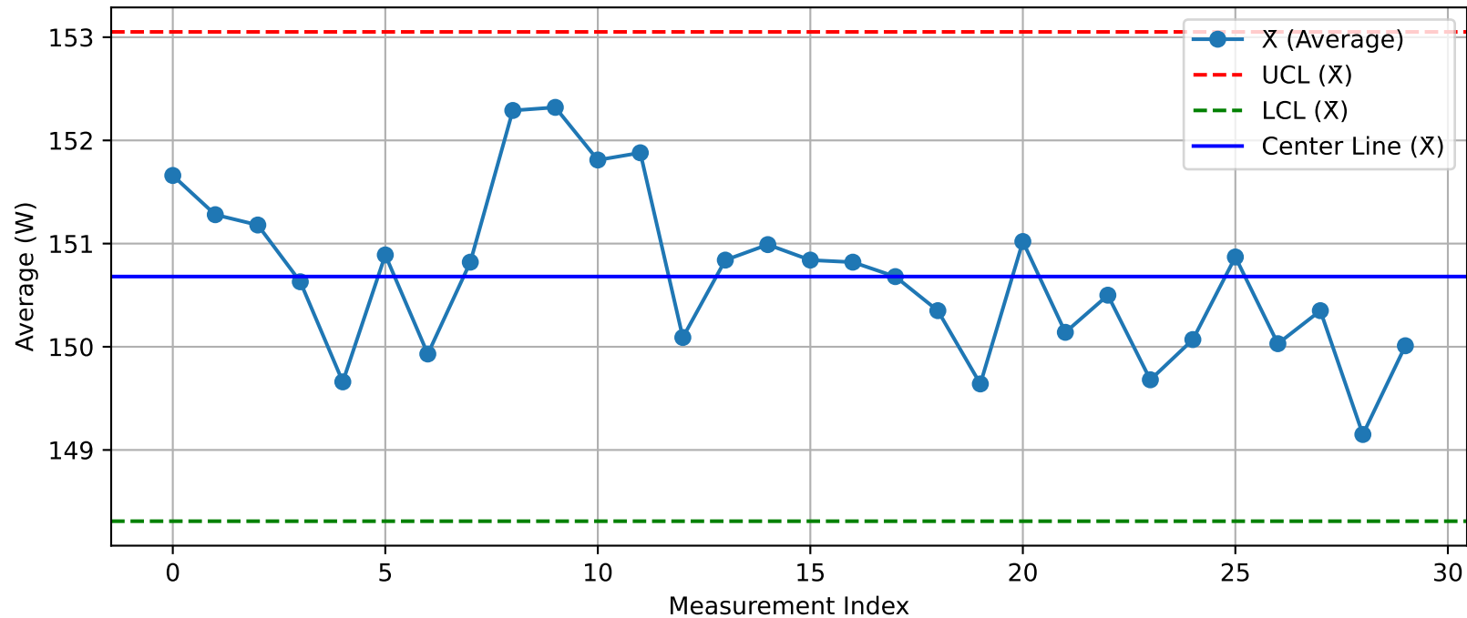
DUT - \bar{X} Chart (T13@Test2_Nuitka.xlsx)
