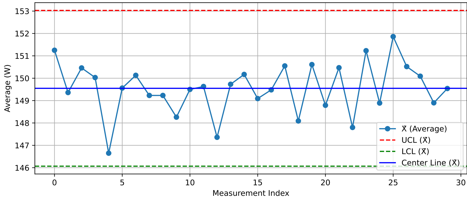
DUT - \bar{X} Chart (T16@Test2.xlsx)
