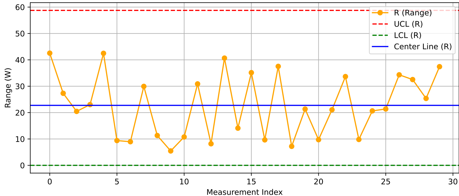
DUT - R Chart (T17@Test1.xlsx)
