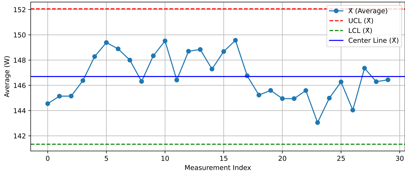
DUT - \bar{X} Chart (T17@Test2.xlsx)
