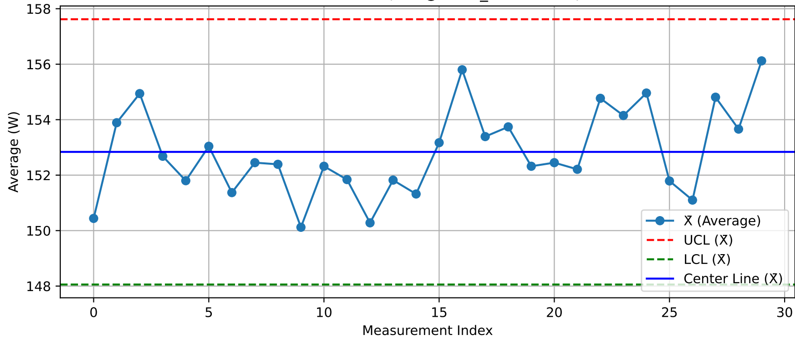
DUT - \bar{X} Chart (T19@Test2_Nuitka.xlsx)
