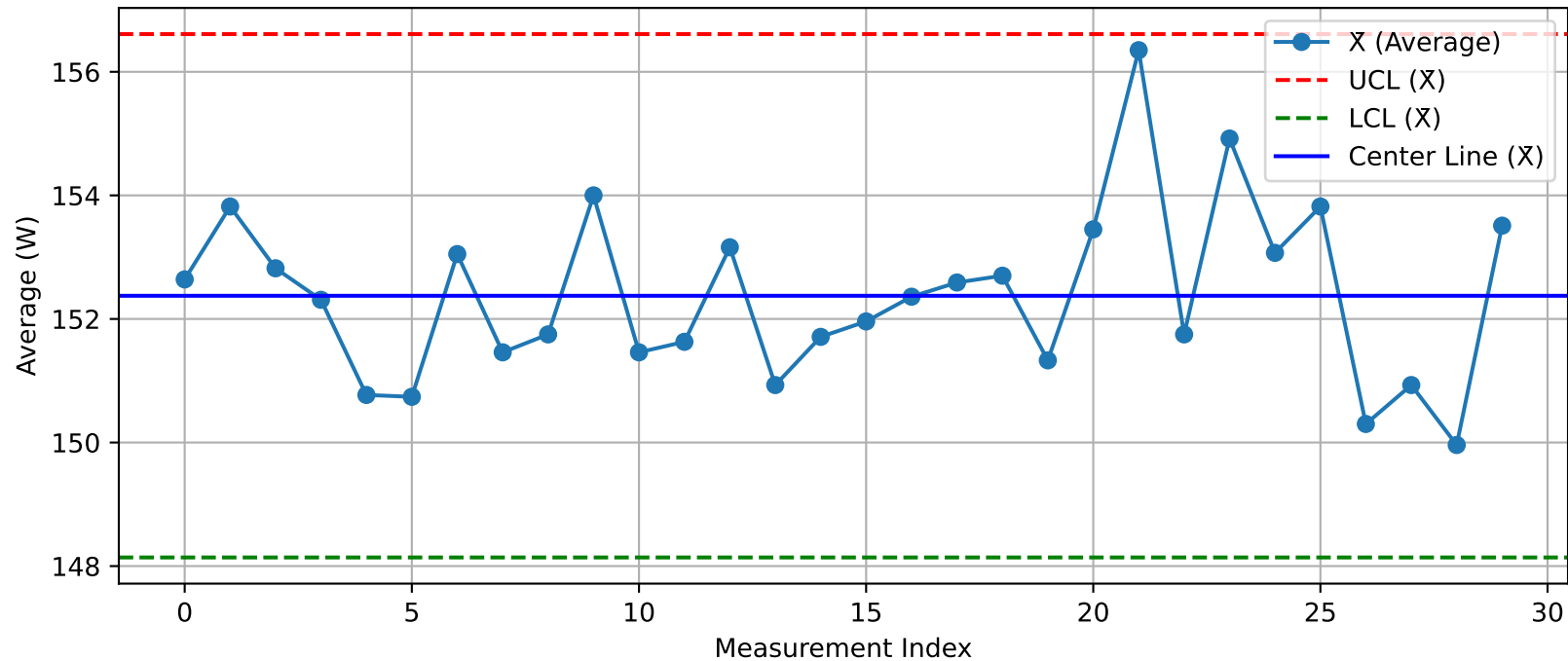
DUT - \bar{X} Chart (T20@Test2_Nuitka.xlsx)
