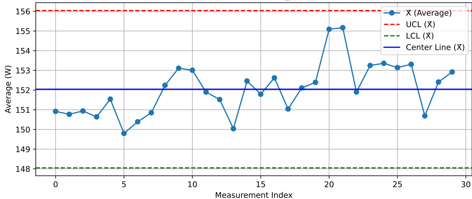
DUT - \bar{X} Chart (T25@Test1_Nuitka.xlsx)
