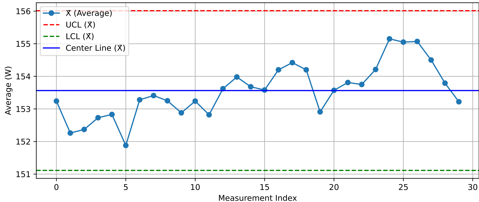
DUT - \bar{X} Chart (T26@Test2.xlsx)
