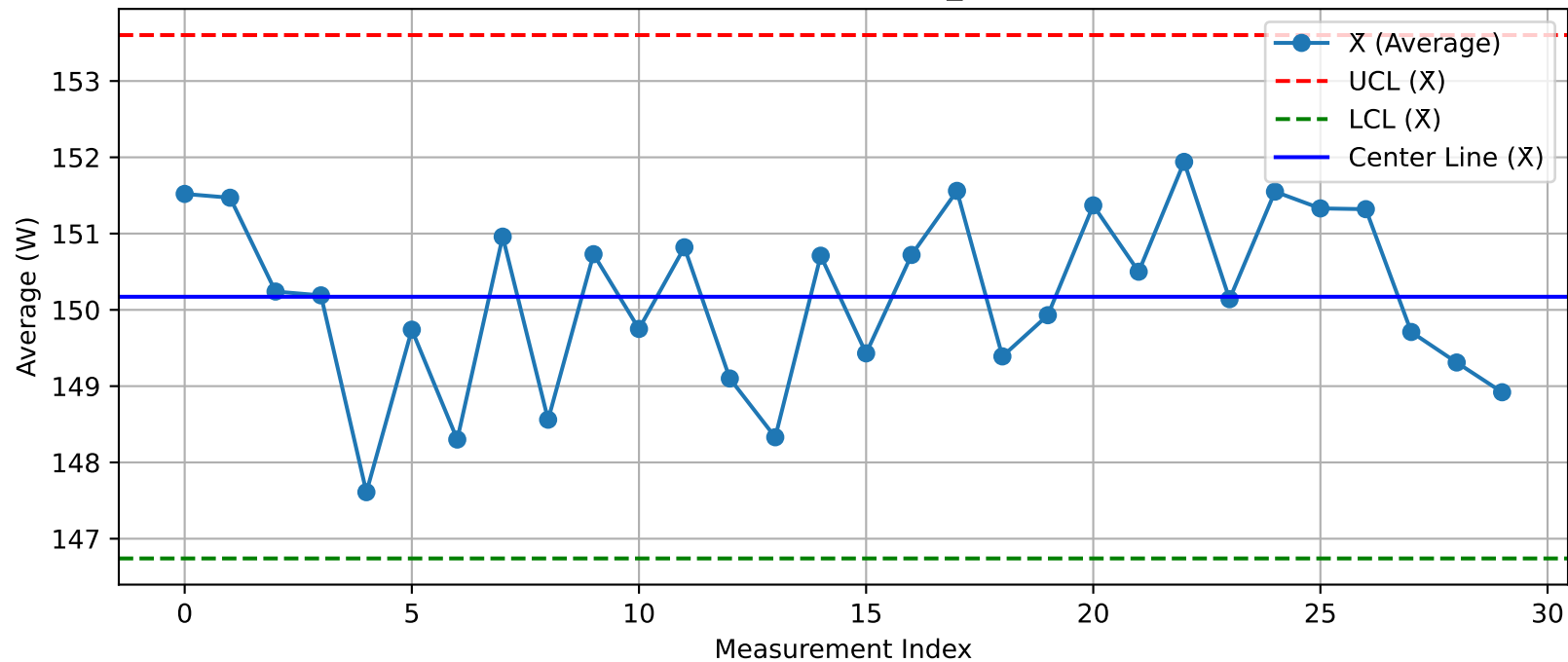
DUT - \bar{X} Chart (T26@Test2_Nuitka.xlsx)
