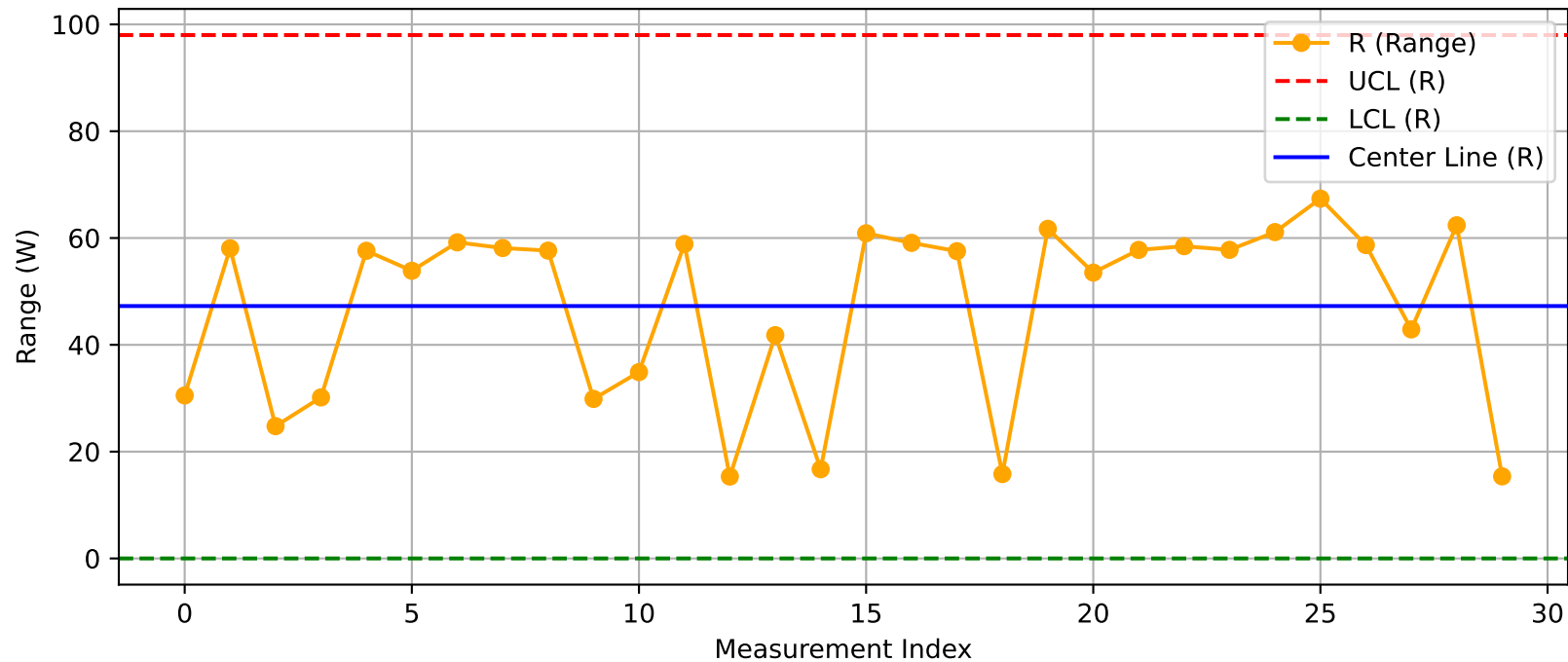
DUT - R Chart (T28@Test1.xlsx)
