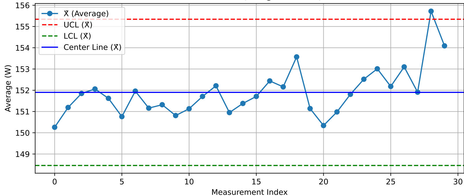
DUT - \bar{X} Chart (T31@Test1.xlsx)
