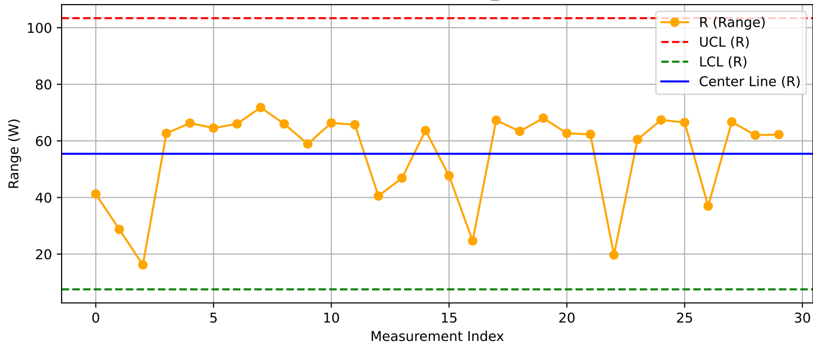
DUT - R Chart (T31@Test2_Nuitka.xlsx)
