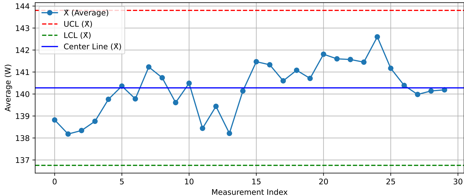
DUT - \bar{X} Chart (T32@Test1.xlsx)
