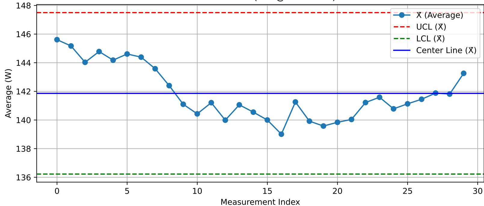
DUT - \bar{X} Chart (T32@Test2.xlsx)
