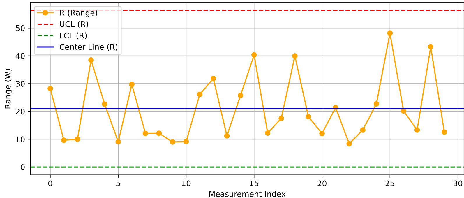
DUT - R Chart (T33@Test1.xlsx)
