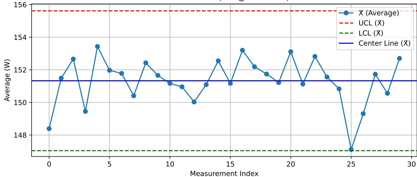
DUT - \bar{X} Chart (T33@Test1.xlsx)
