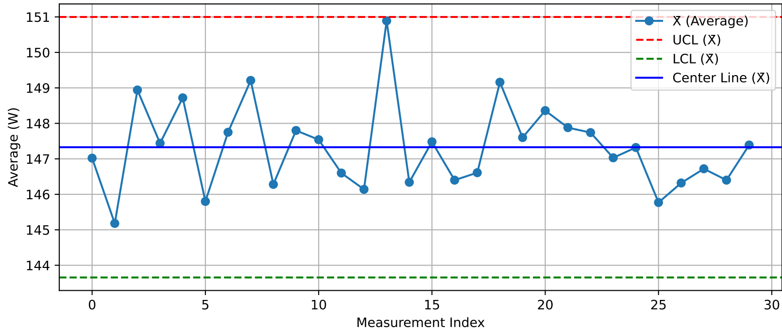
DUT - \bar{X} Chart (T33@Test2_Nuitka.xlsx)
