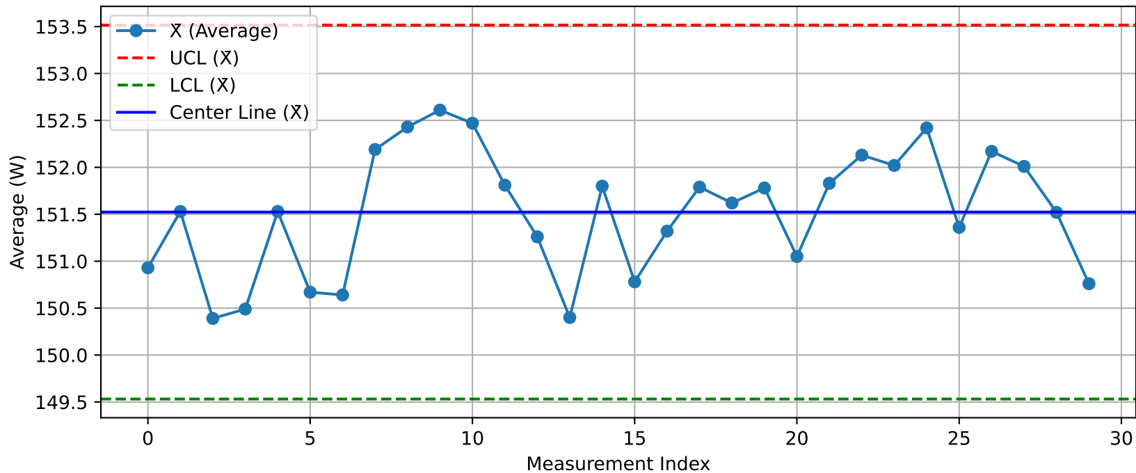
DUT - \bar{X} Chart (T36@Test1.xlsx)
