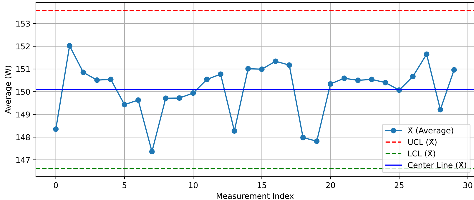
DUT - \bar{X} Chart (T36@Test2_Nuitka.xlsx)
