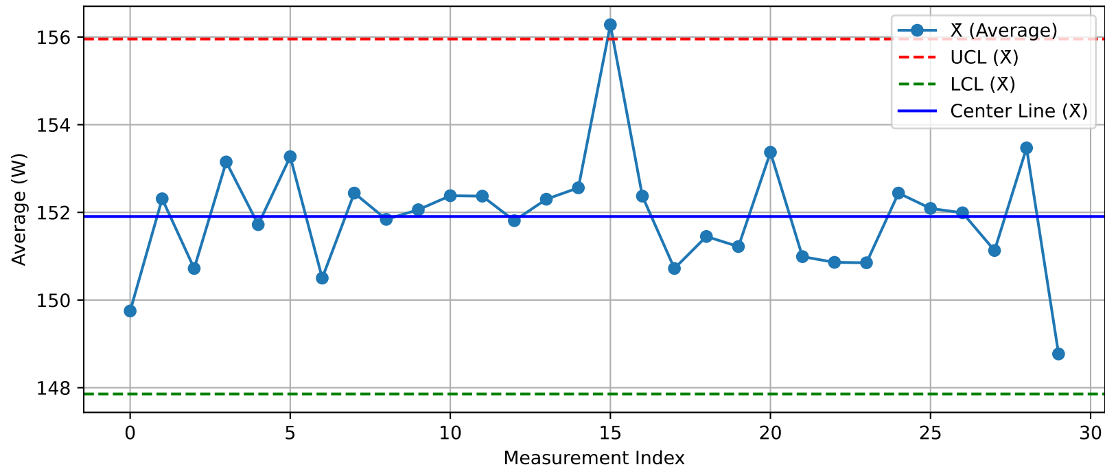
DUT - \bar{X} Chart (T44@Test1.xlsx)
