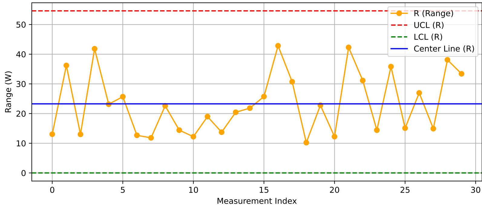
DUT - R Chart (T49@Test2.xlsx)
