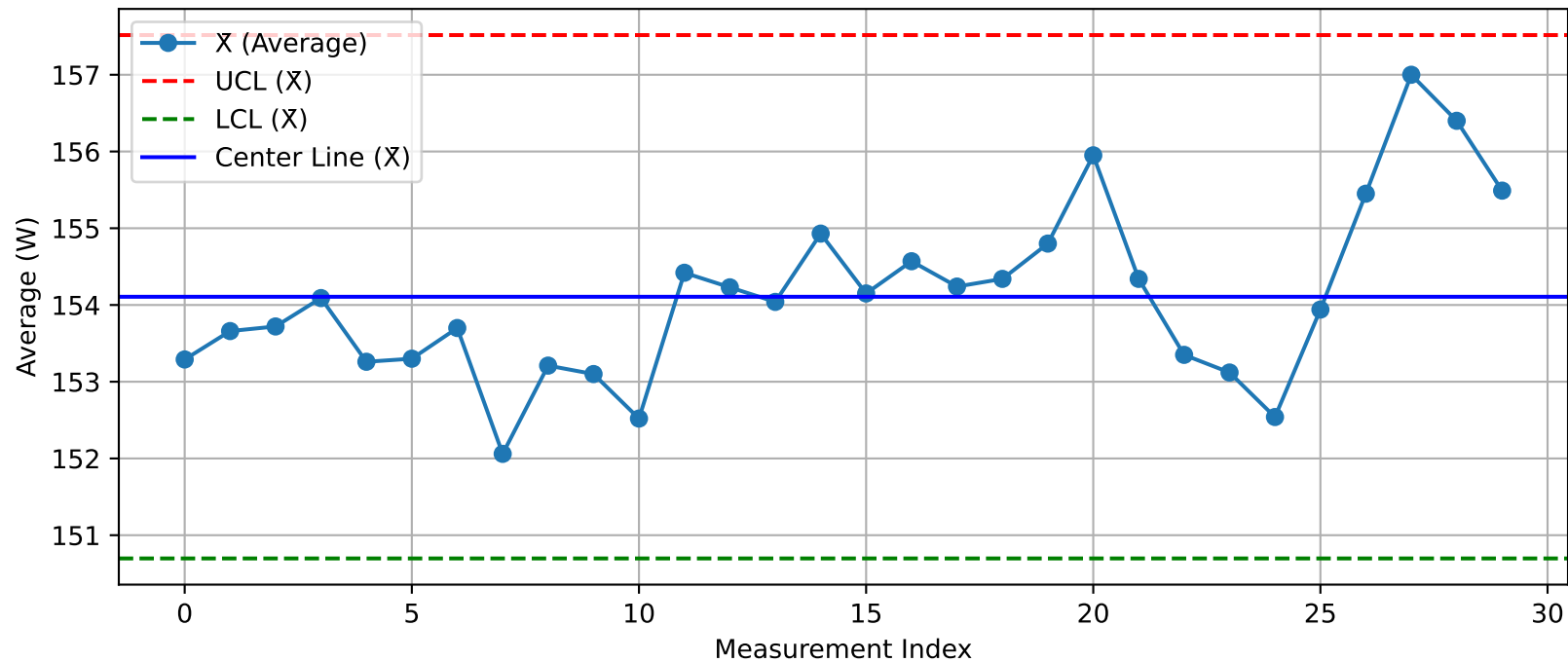
DUT - \bar{X} Chart (T4@Test1.xlsx)
