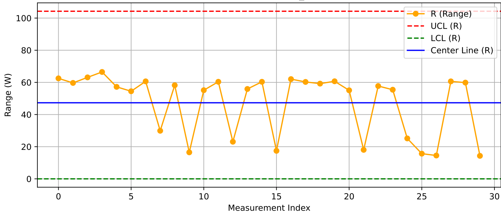
DUT - R Chart (T4@Test1_Nuitka.xlsx)
