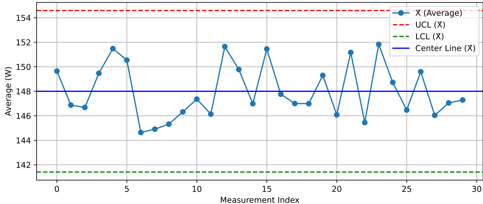
DUT - \bar{X} Chart (T50@Test2_Nuitka.xlsx)
