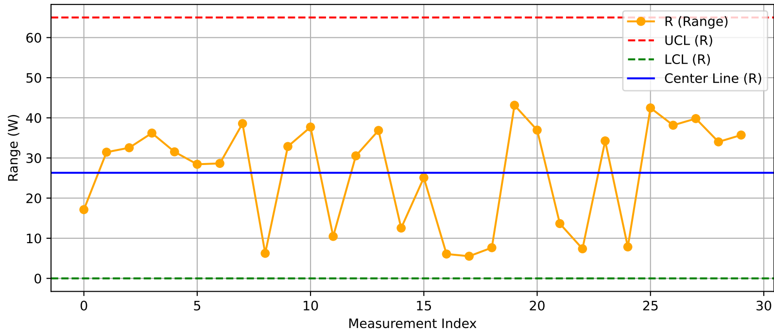
DUT - R Chart (T5@Test1.xlsx)
