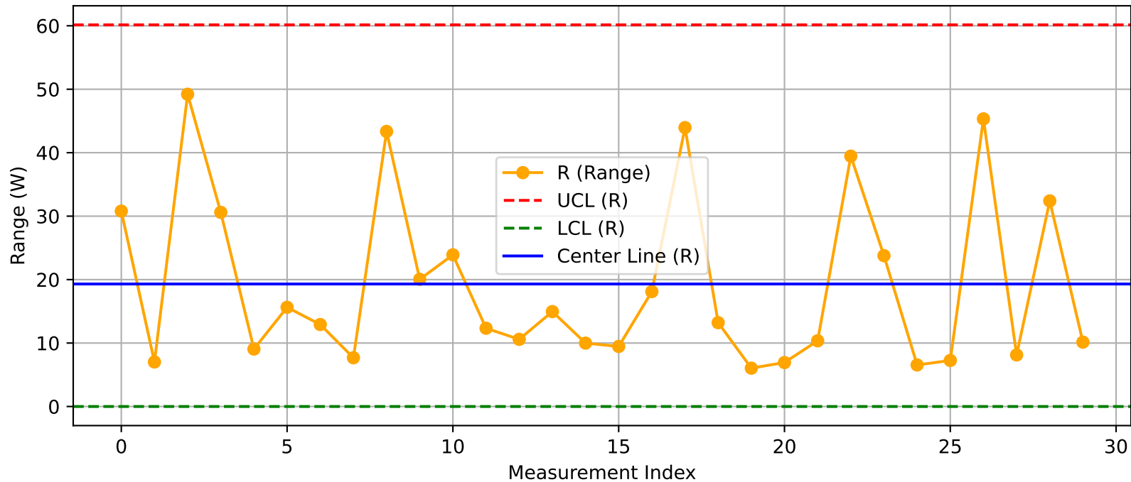
DUT - R Chart (T5@Test2_Nuitka.xlsx)
