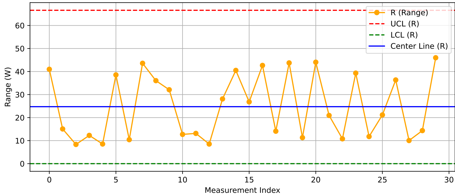
DUT - R Chart (T7@Test2.xlsx)
