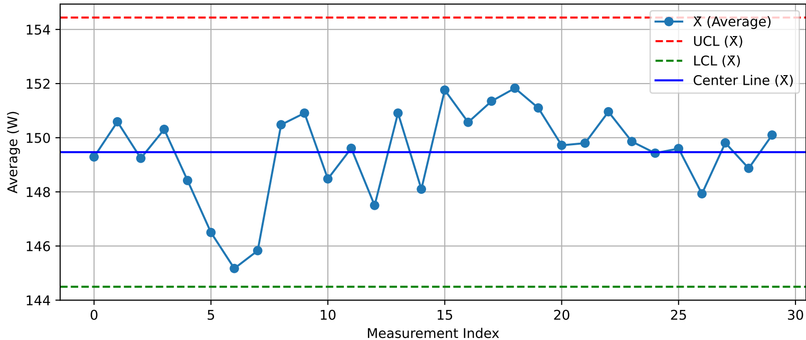
DUT - \bar{X} Chart (T7@Test2_Nuitka.xlsx)
