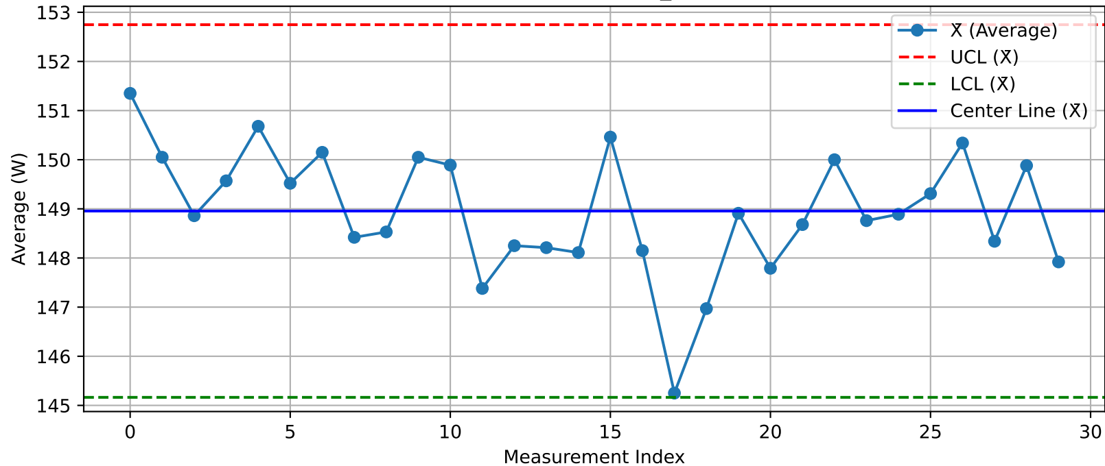
DUT - \bar{X} Chart (T8@Test2_Nuitka.xlsx)
