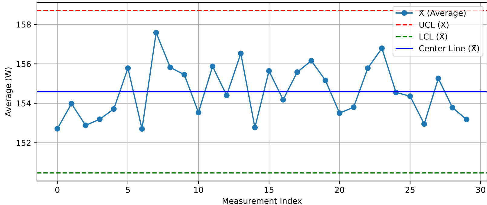
DUT - \bar{X} Chart (T9@Test1.xlsx)
